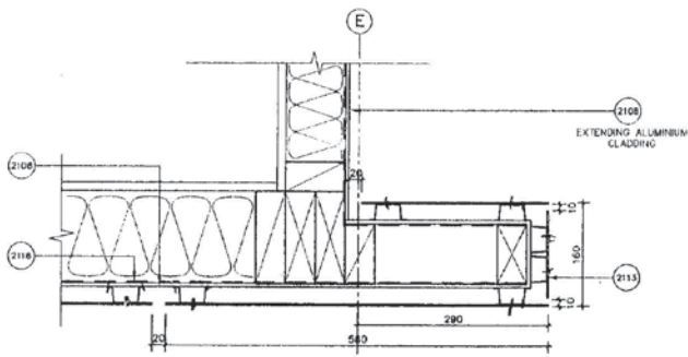
A(21)1203 WALL DETAIL 1:5 PLAN
